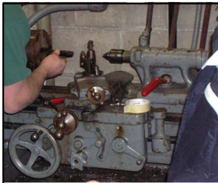
Setting up a steering shaft to drill off old threads and make new ones.
