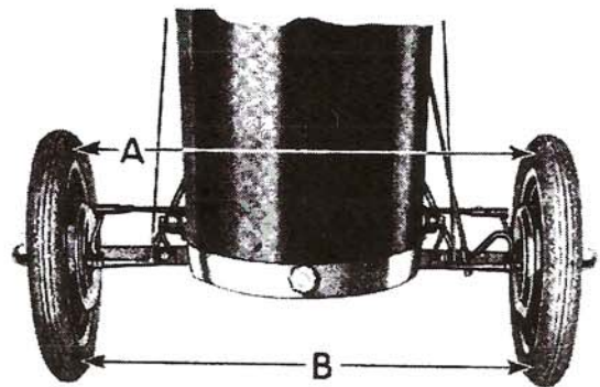
Adjust "B" Tow-In 1/8" Narrower Than "A"
